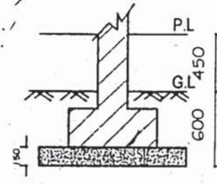
FOUNDATION DETAIL
